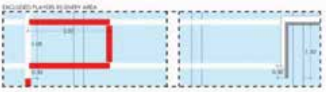
Suits current FINA standard: 1080mm player re-entry area
