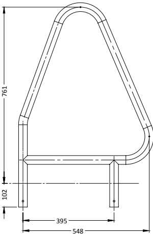
Triangle Grab Rail (SR-6S Standard/SR-6F Flanged)
