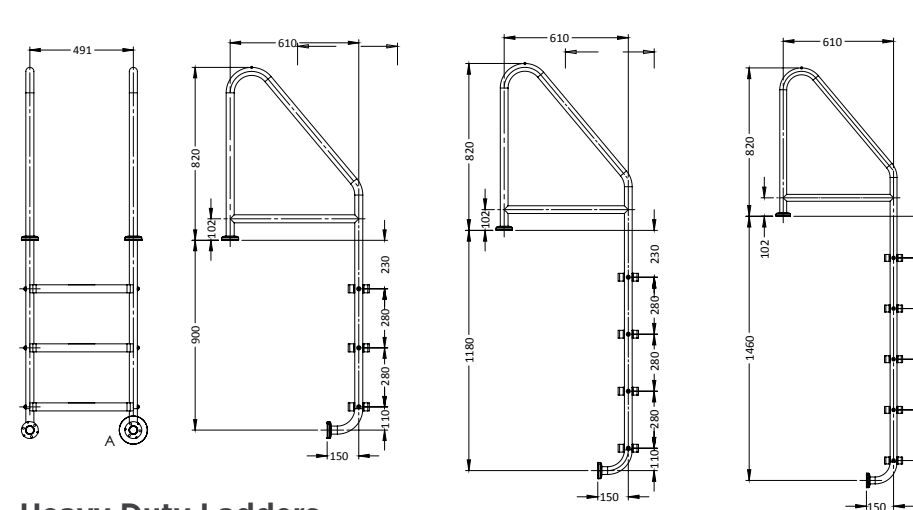
Heavy Duty Ladders (SR-XS-3 Three-Step Ladder Flanged Top & Bottom/ SR-XS-4 Four-step Ladder Flanged Top & Bottom)/SR-XS-5 Five-Step Ladder Flanged Top & Bottom)
