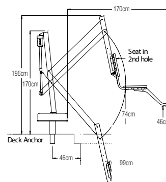
EXTENDED REACH SIDE VIEW
