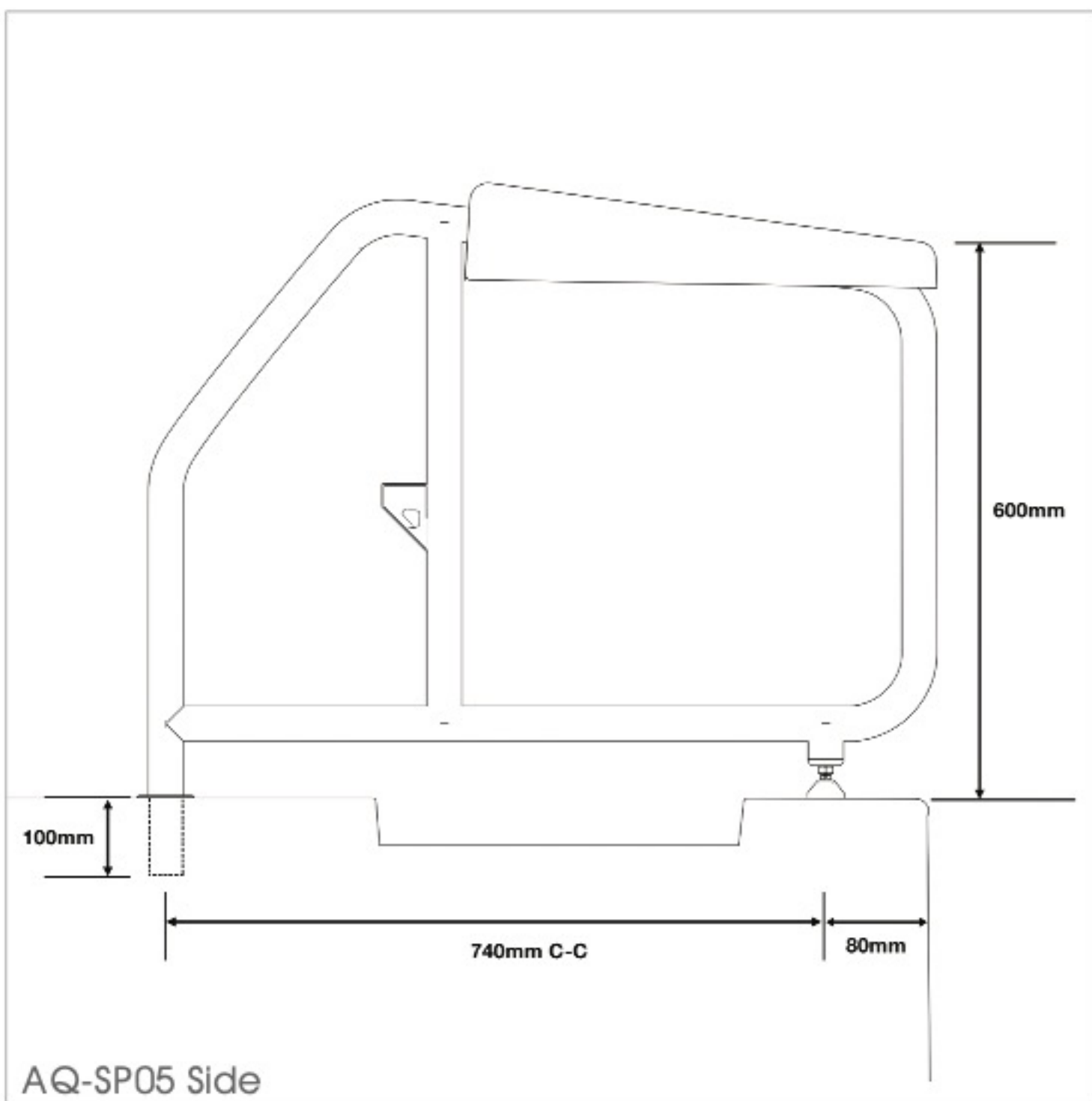
AQ-SP05-C with Blue Top
